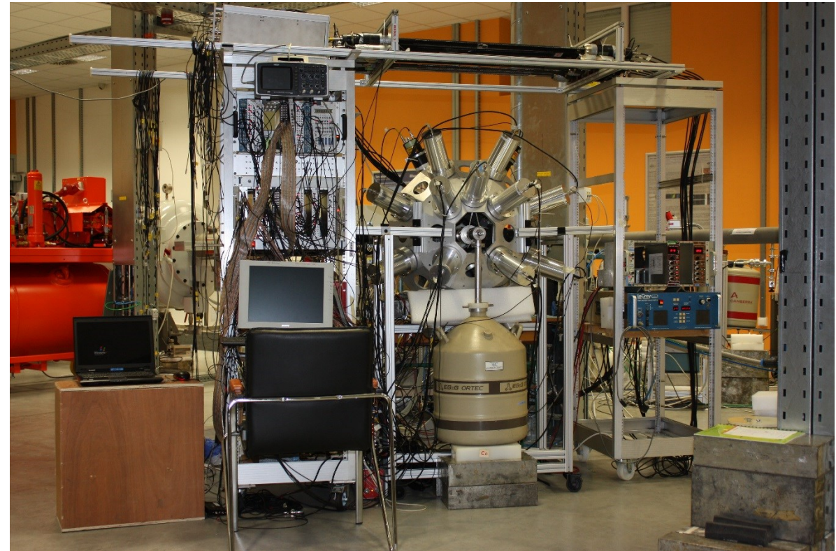
\gamma -spectrometer with twelve, 3"x3" and two 3.5"x6" LaBr 3 detectors
